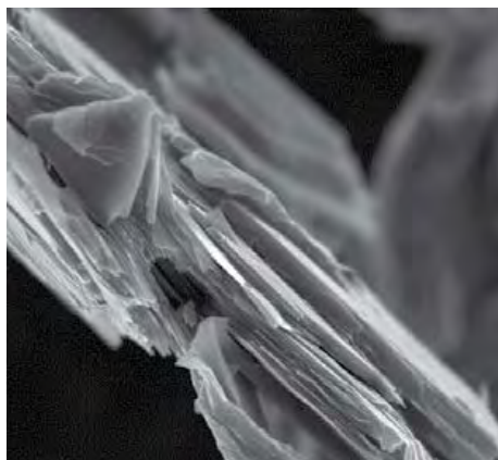
Figure 2: Scanning electron microscopy of borate treated graphite
