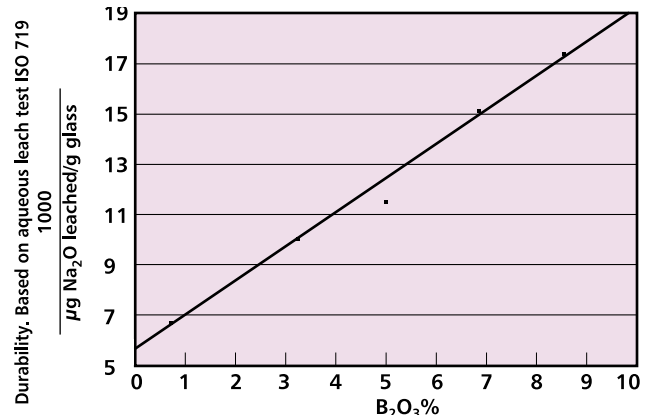
Effect of B 2 O 3 on Insulation Fiberglass Durability
